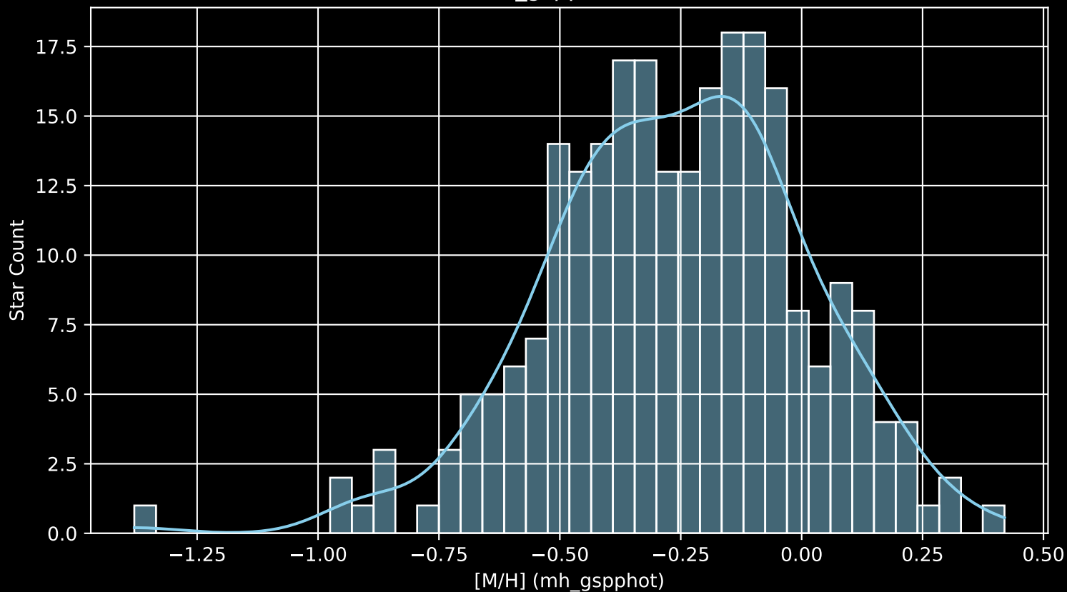
GALAH DR4 Field: [7202] [M/H] (mh_gspphot) (n= 246)
