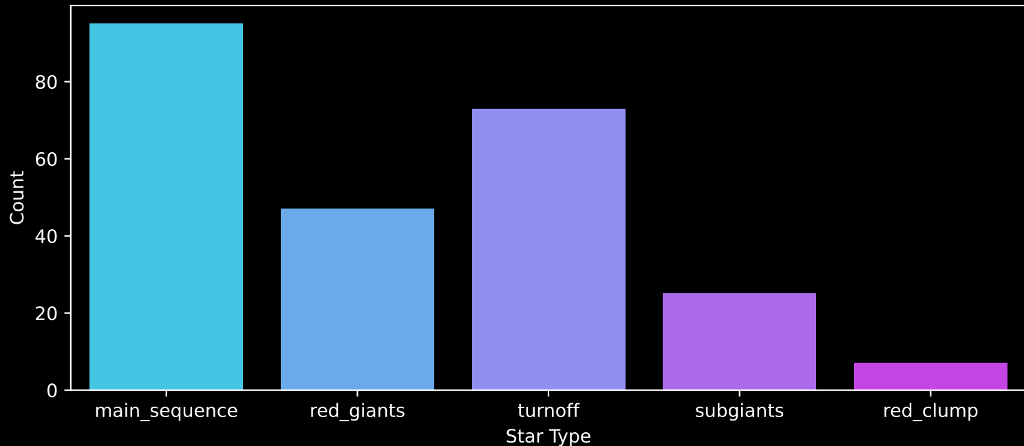
GALAH DR4 Field: [7202] Count plot of Star Type
