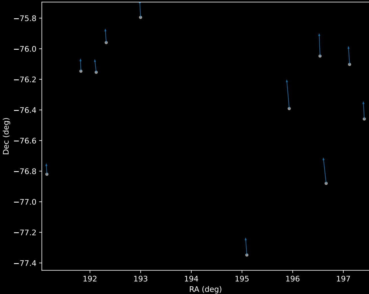
GALAH DR4 Cluster 0 Proper Motion Vectors (n=11)
