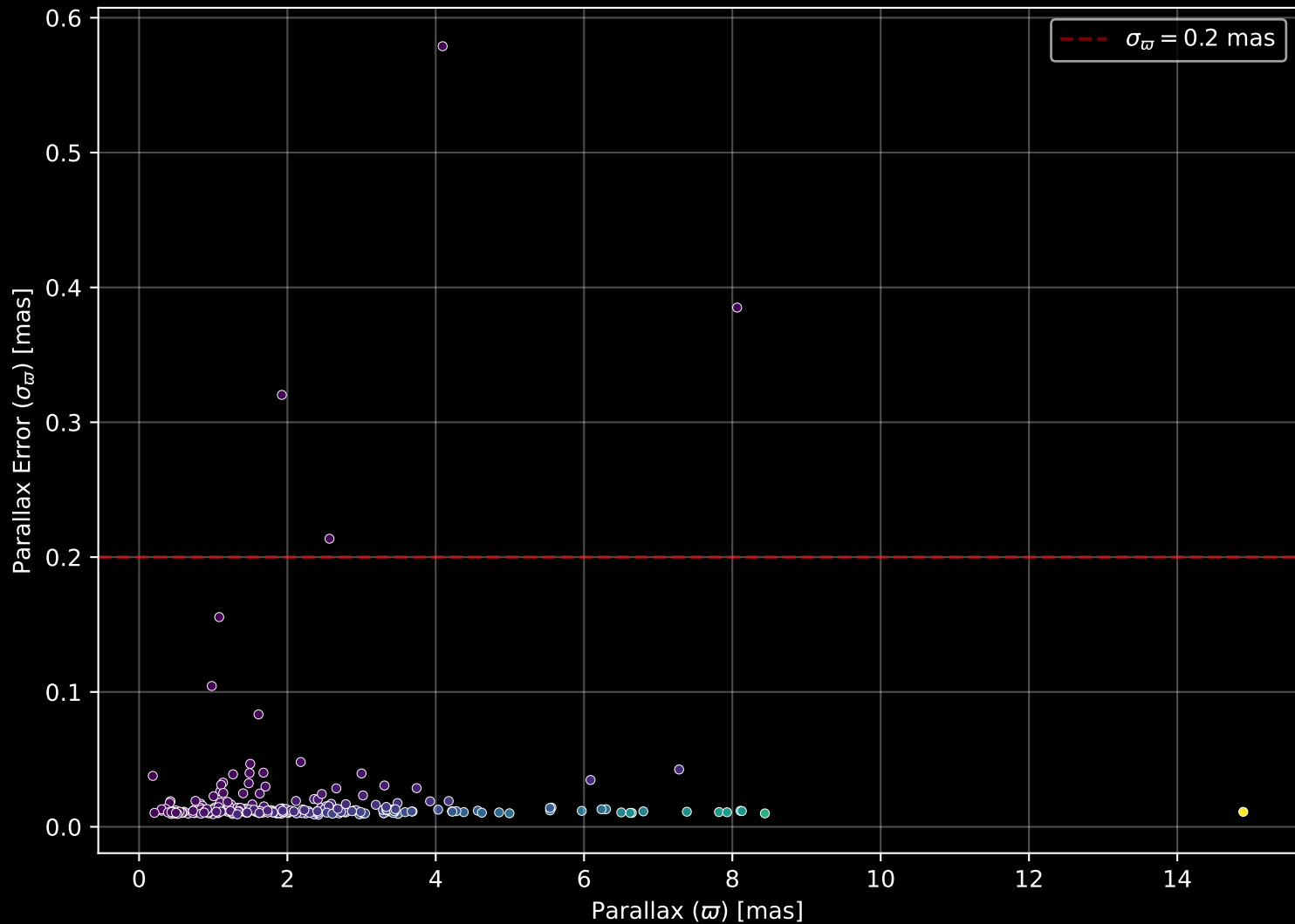
GALAH DR4 Field: [7202] Parallax Quality (n= 247)
