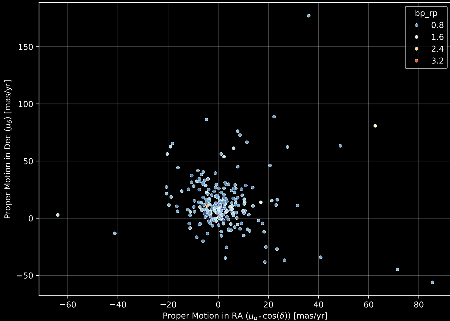
GALAH DR4 Field: [7202] Proper Motion Diagram (n= 247)
