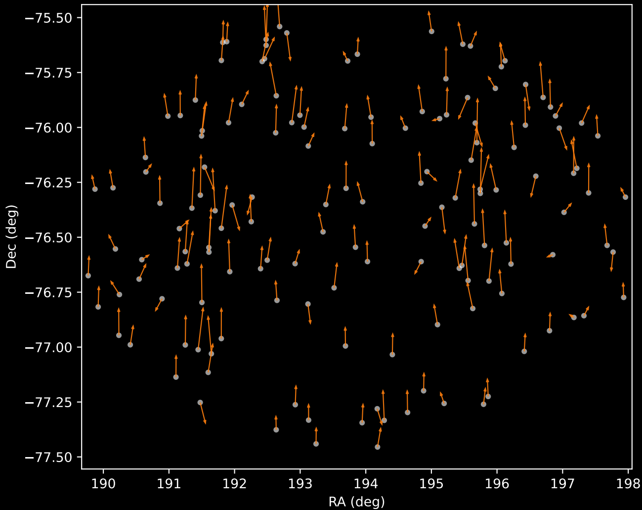
GALAH DR4 Cluster 2 Proper Motion Vectors (n=149)
