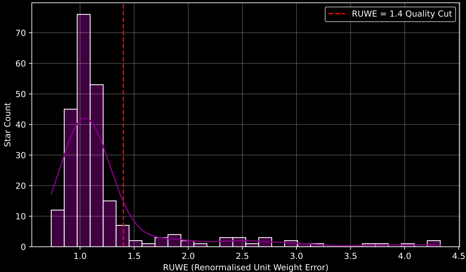
GALAH DR4 Field [7202] RUWE Distribution (n= 240)
